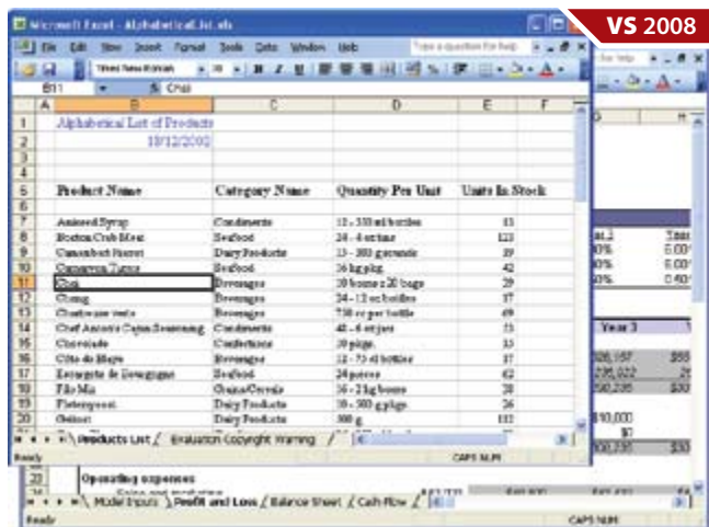
Aspose.Cells
