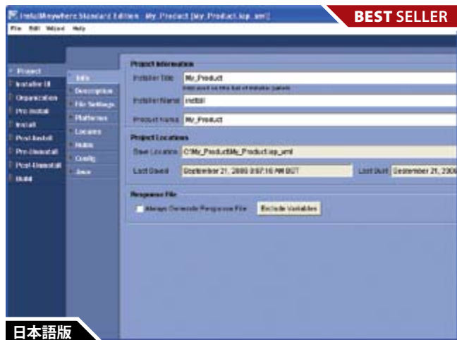
InstallAnywhere
