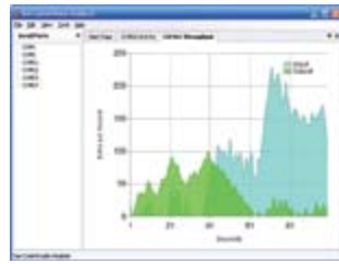
Sax CommStudio
