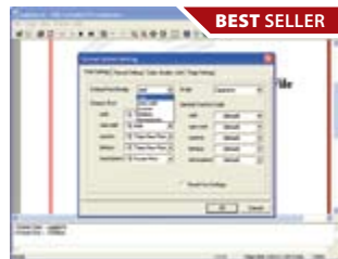
XSL Formatter
