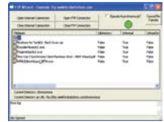
FTP Wizard
